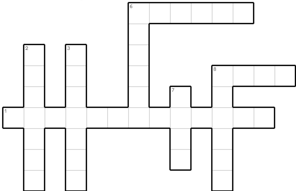
Parallelogram
