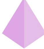
Pyramide
