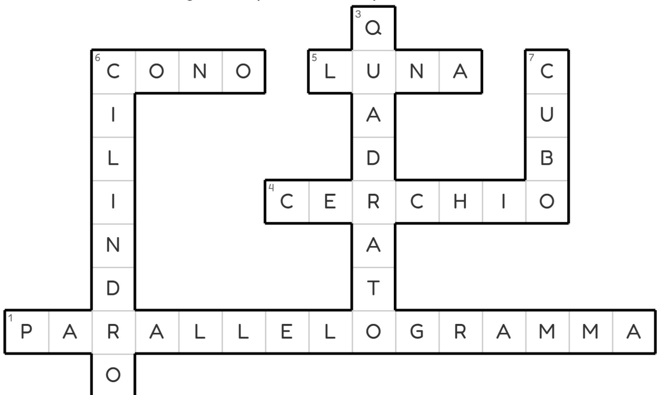
Parallelogram
