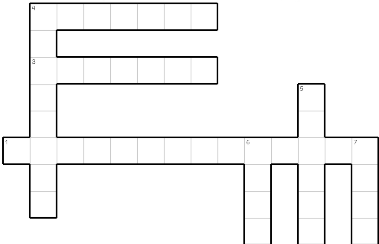
Parallelogram
