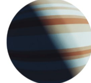
Neptune
