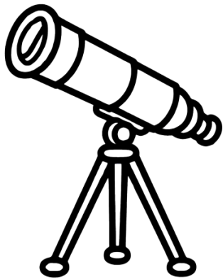
telescope
