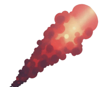
comet
