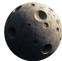
asteroid
