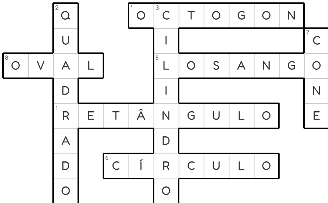
Rectangle
