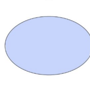
Oval
