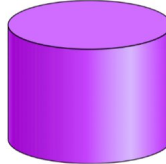
Cylinder
