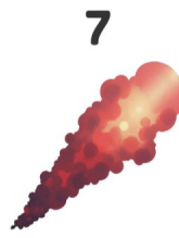
Comet
