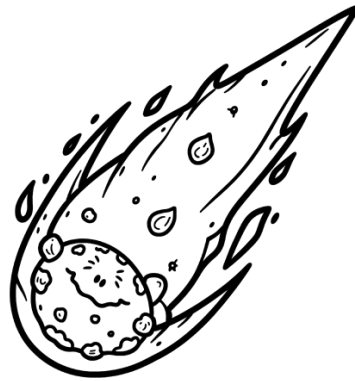
meteor
